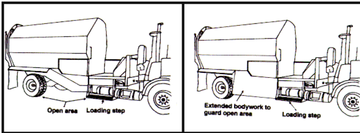
Figure 2. Typical side-loading refuse collection vehicle with extended bodywork to guard the open area between the loading step and the rear wheels.
